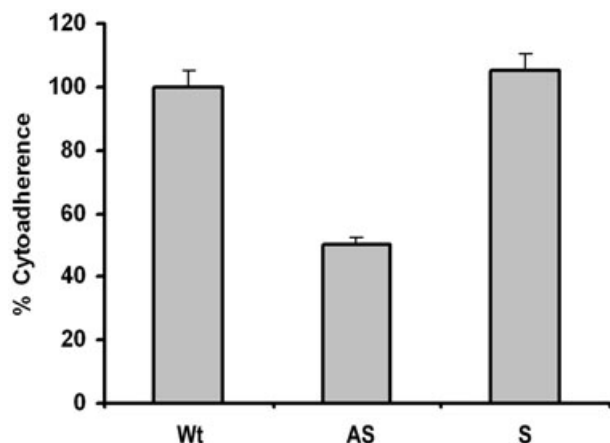
Fig. 6. Antisense (AS) transfected T. vaginalis organisms have lower levels of adherence to immortalized MS-74 vaginal epithelial cells compared to sense transfected (S) and wild type (Wt) trichomonads. The extent of adherence by Wt parasites was normalized to 100% for comparative purposes, as before (Arroyo et al. , 1992; Garcia et al. , 2003). The results are the average and standard deviations from four different experiments. Each experiment was performed with quadruplicate samples.
