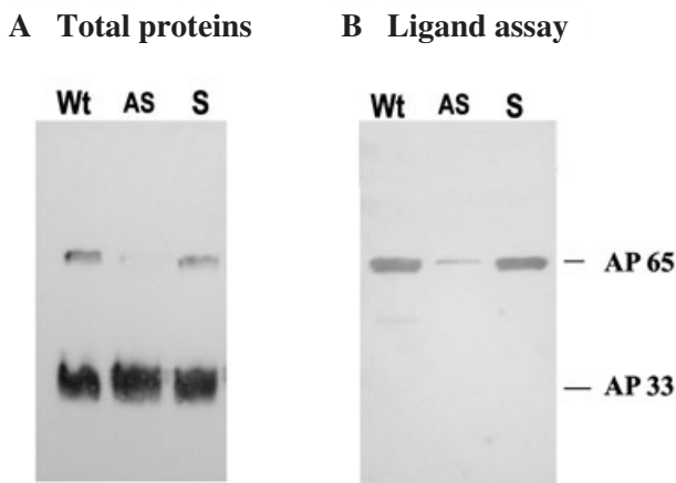
Fig. 3. Immunoblots with specific mAb DM116 detecting the amount of AP65 in total protein preparations (A) and bound to HeLa cells in a ligand assay (B) from equal numbers of S and AS transfected trichomonads compared to control Wt organisms.
