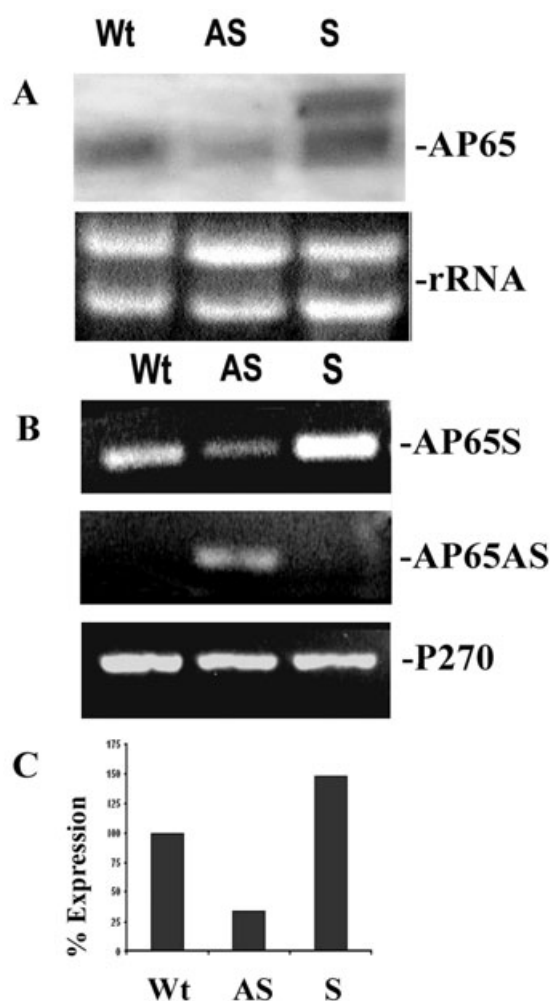
Fig. 2. Levels of ap65 mRNA in antisense (AS) transfected trichomonads is less than transcript in the sense (S) and wild type (Wt) organisms.
