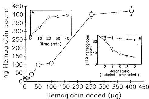
FIGURE 3. Concentration-dependent binding of ^{125}\text{I} -labeled hemoglobin to T. vaginalis NYH 286. The time course binding of ^{125}\text{I} -labeled hemoglobin to T. vaginalis NYH 286 is shown in inset A under conditions described in Materials and Methods. Inset B shows a representative competition experiment with increasing amounts of unlabeled hemoglobin (O) or lactoferrin (●). Results are of quadruplicate samples of three experiments.
