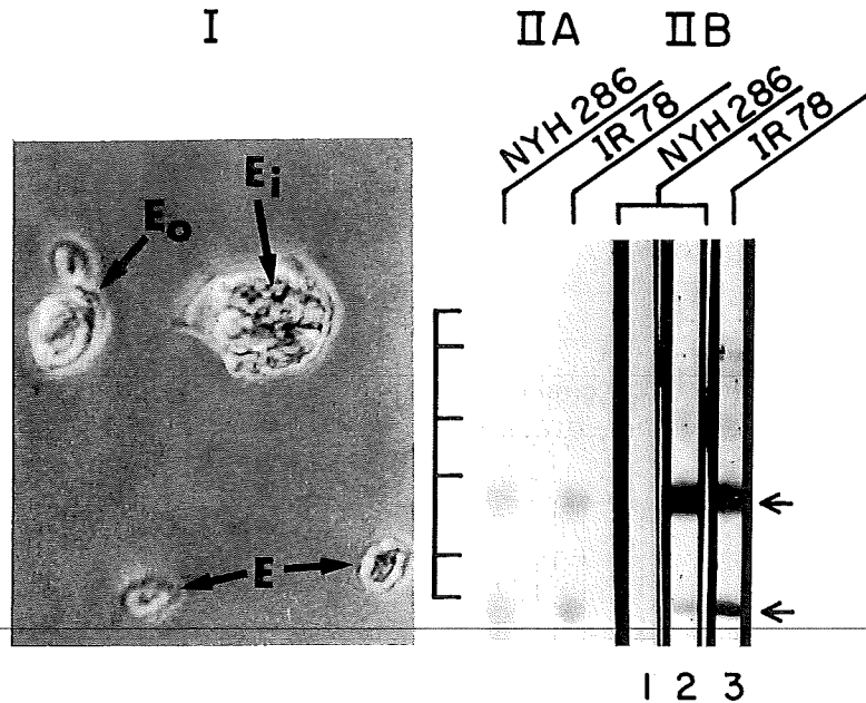
FIGURE 1. Internalization of glutaraldehyde-fixed erythrocytes by live parasites of T. vaginalis isolate NYH 286 (I) and identification of erythrocyte-binding trichomonad surface proteins (II). (I) E_o refers to adherent erythrocytes outside the organisms vs. internalized erythrocytes ( E_i ) and unbound erythrocytes in suspension ( E ). (IIA) Autoradiograms show binding to fixed erythrocytes of two trichomonad proteins (arrows) from a detergent extract of iodinated organisms. Molecular weight markers were from BioRad Laboratories (Richmond, CA). (IIB) The reaction of undiluted mouse antiserum to the 27,500 EBP of isolate NYH 286 with nitrocellulose blots of proteins from the ligand assay (see Materials and Methods) of isolates NYH 286 (lane 2) and IR 78 (lane 3). The reaction of prebled mouse serum with a duplicate blot of NYH 286 EBPs is shown in lane 1. Antiserum to the 12,500 EBP was identical by immunoblots with that shown for antiserum to the 27,500 EBP (lanes 2 and 3).
